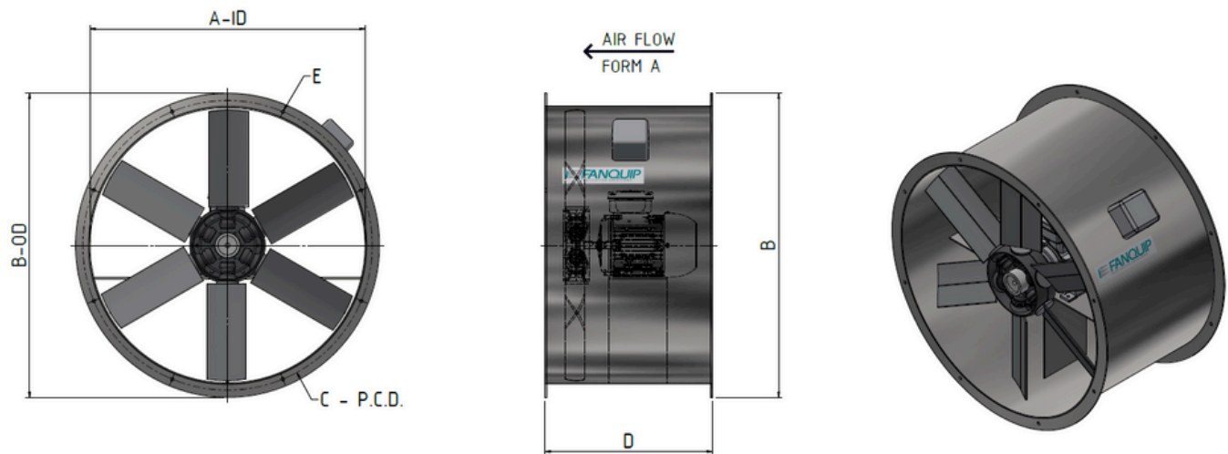
Product dimensions.
