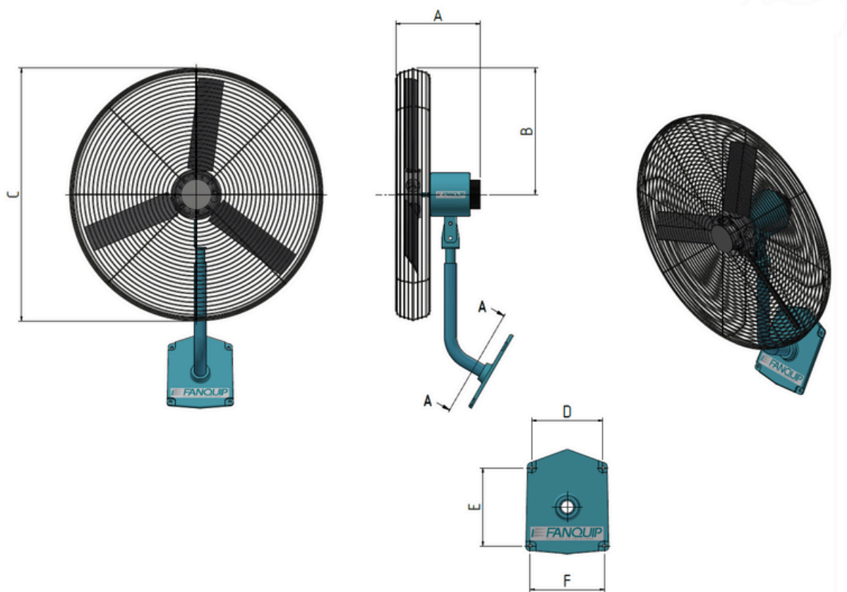
Product dimensions.
